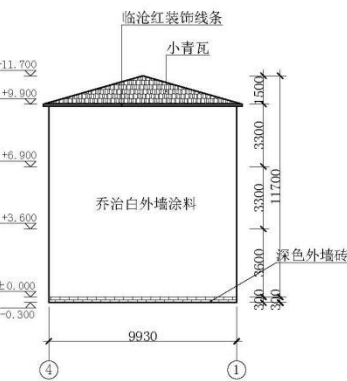
D—A 轴立面图1:200
